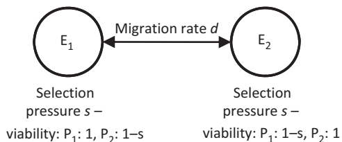
Fig. 1 A simple formal model of selection-based and detection-based effects. A population with two phenotypes P_1 and P_2 is split into two subpopulations living in environments E_1 and E_2 under selection pressure s against nonmatching phenotypes, and migrating between patches at rate d .
